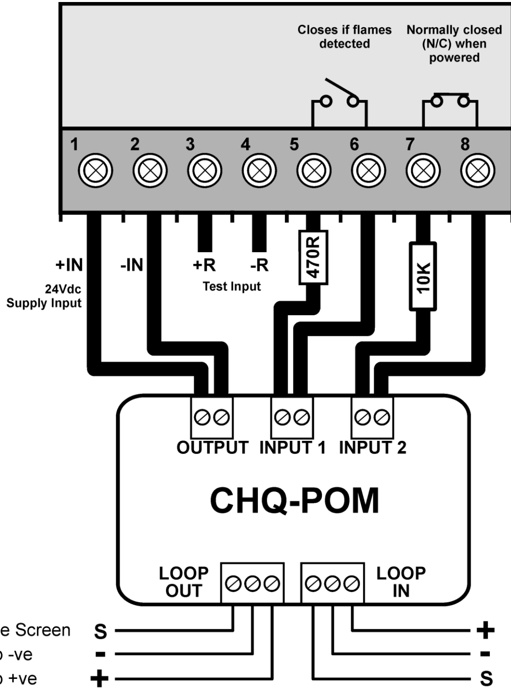
Fig 12 Connection Diagram using a CHQ-POM Powered Output Module
