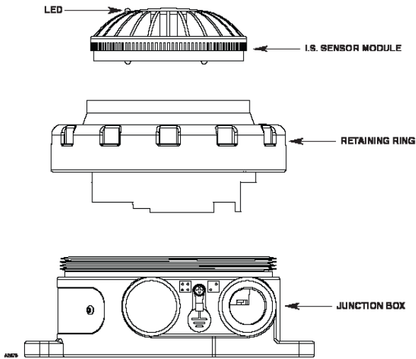
Figure 1—U5015 Components
