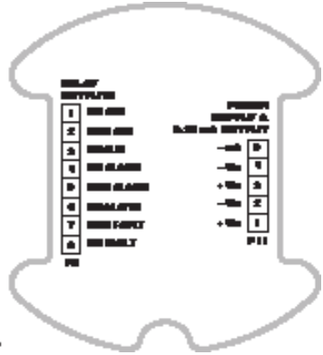
Figure 9—Wiring Terminals
