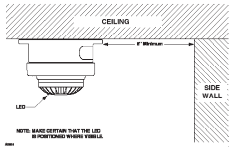
Figure 5—U5015 Ceiling Mount
